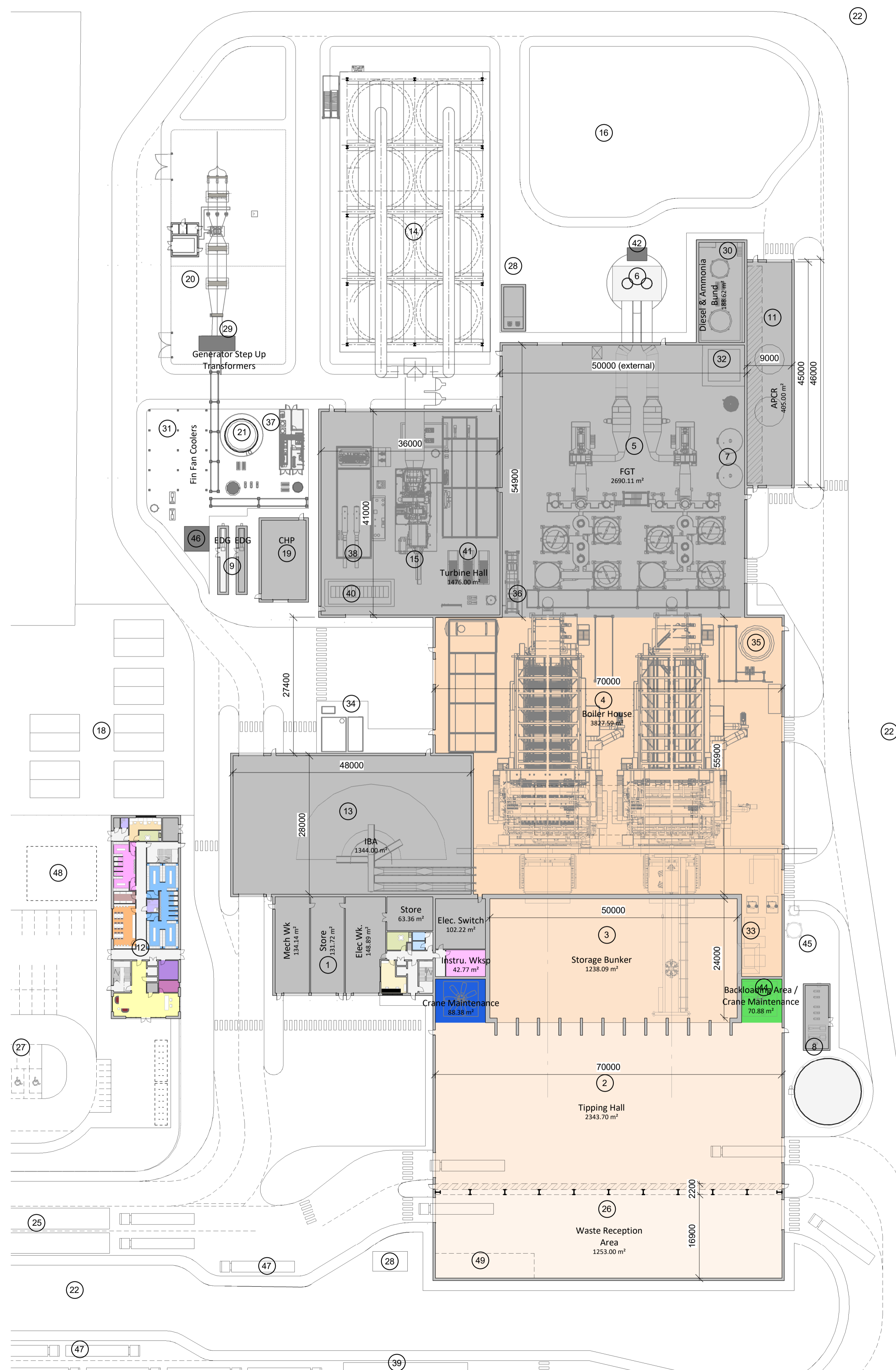
GA Plan - Level 00
