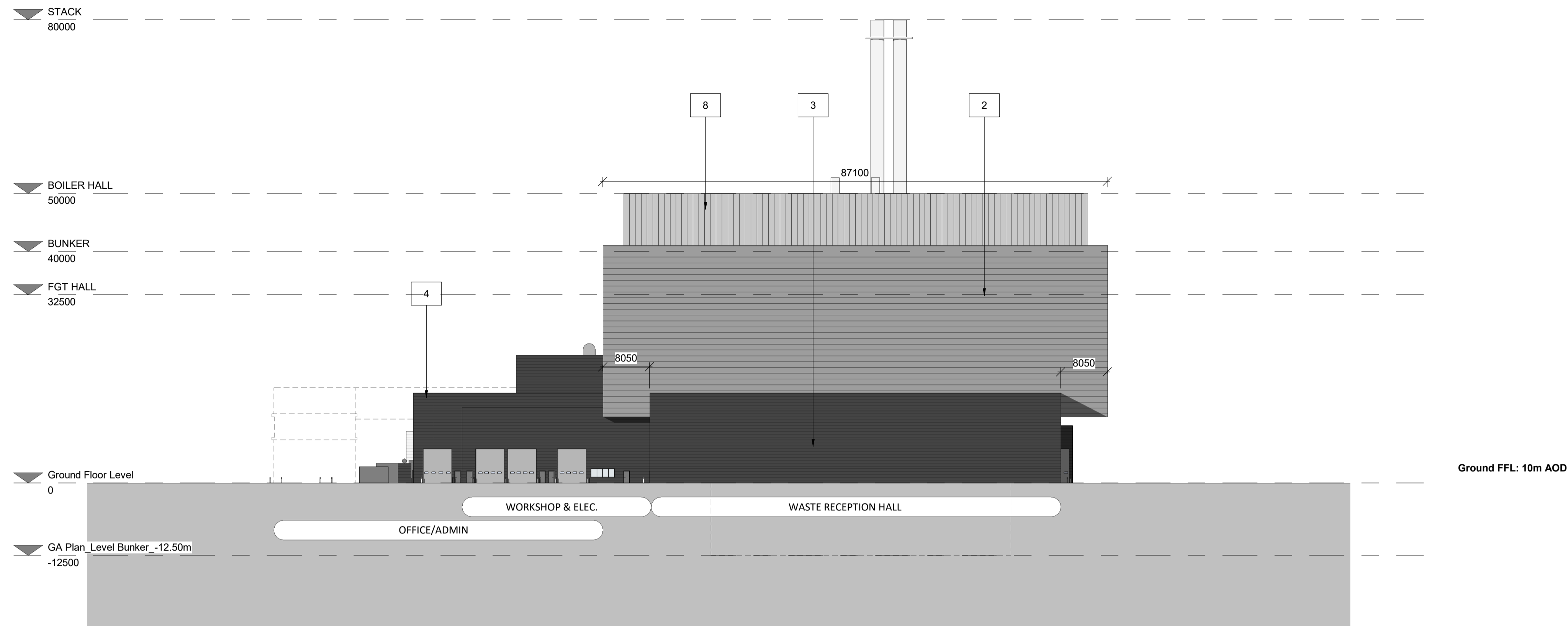
SOUTH_Elevation
